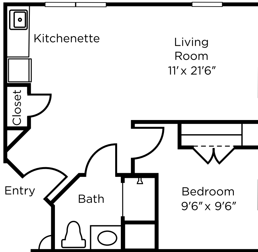
ALU One Bedroom Apartment Type 4 555 sq. ft.
